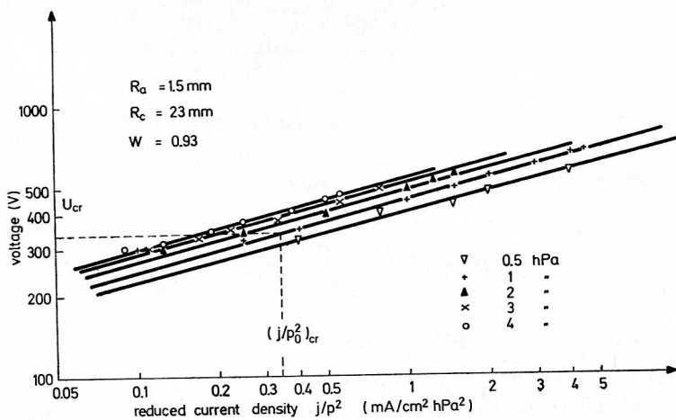
Fig. 3. The cathode fall-reduced current density dependence in log-log scale
