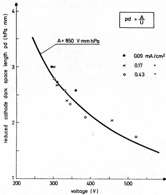
Fig. 5. Reduced cathode dark space length as a function of the cathode fall
